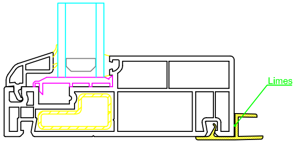
Clipsbar U-Liste, for 10mm plade Notprofil 3
